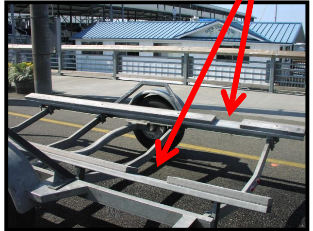
Full bunks with cut outs
